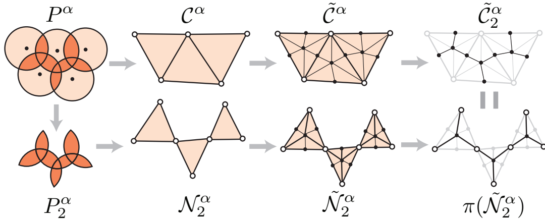
Figure 3: We transform the collection of balls in two different ways to get equivalent complexes, \tilde{C}_k^\alpha (top) and \pi(\tilde{N}_k^\alpha) (bottom) for k = 2 .
